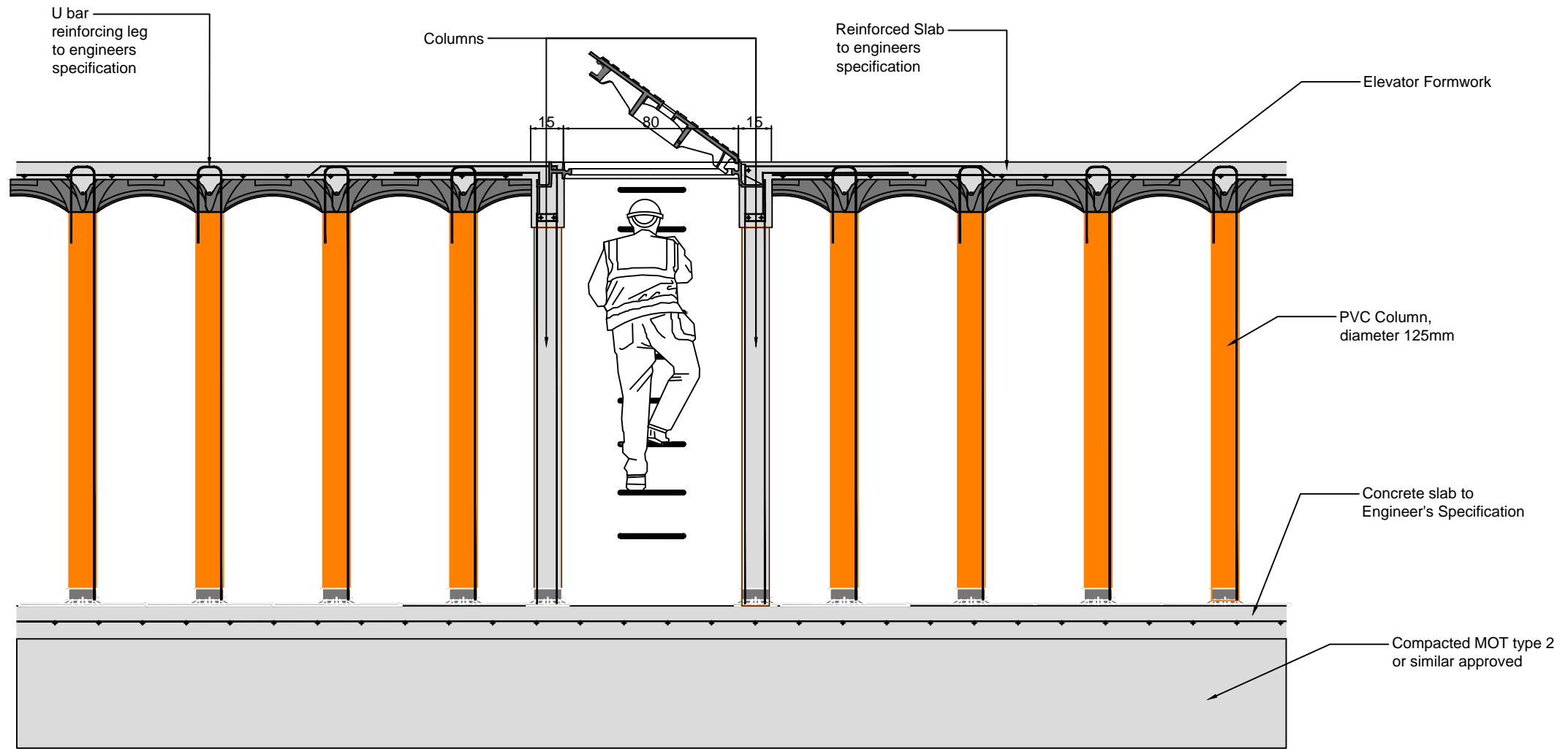
Manhole support columns : schematic design, structural and execution details to be defined.
